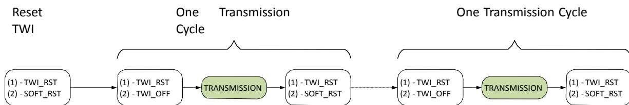
Figure 16. T119 Operation Flow with TWI
