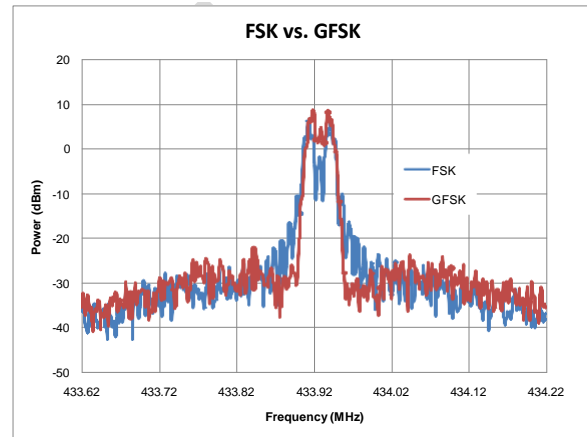
Figure 5. FSK/GFSK Spectrum, SR = 9.6 ksp/s, F_{DEV} = 15 kHz
