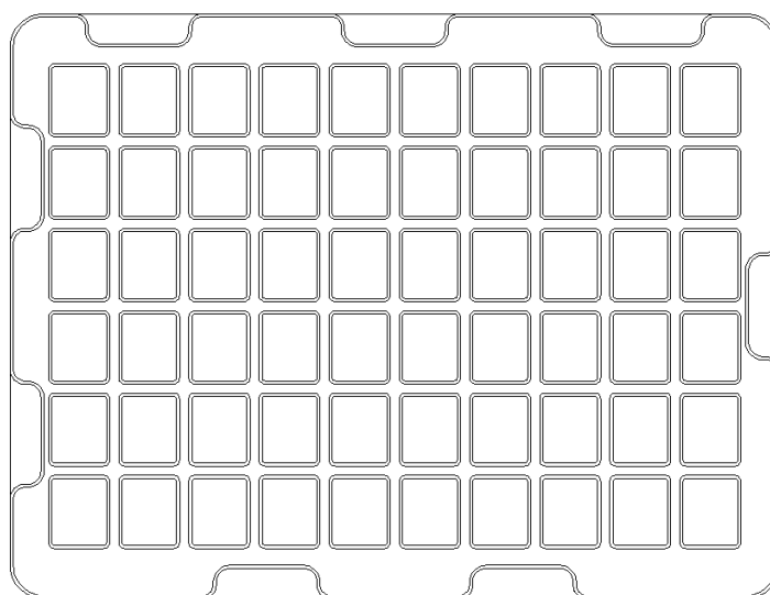
Figure 24. Package Outline Drawing
