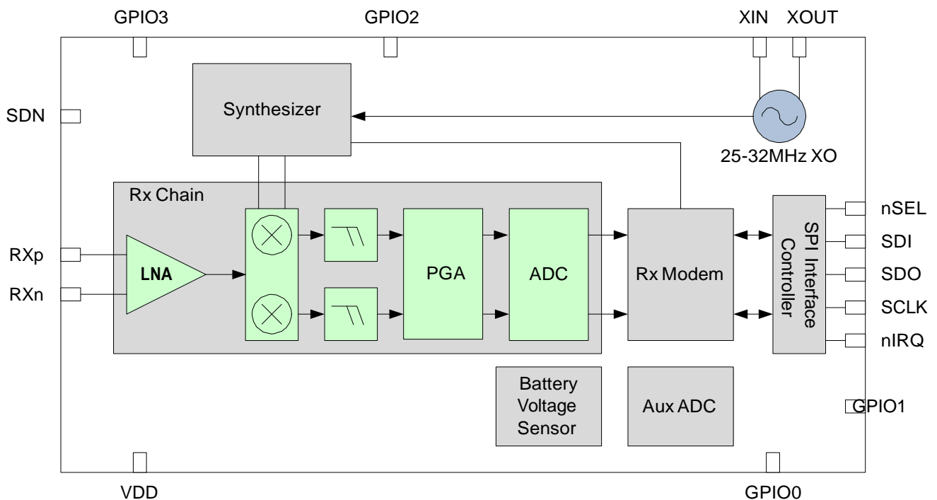
Figure 2. HC4355 Functional Block Diagram
