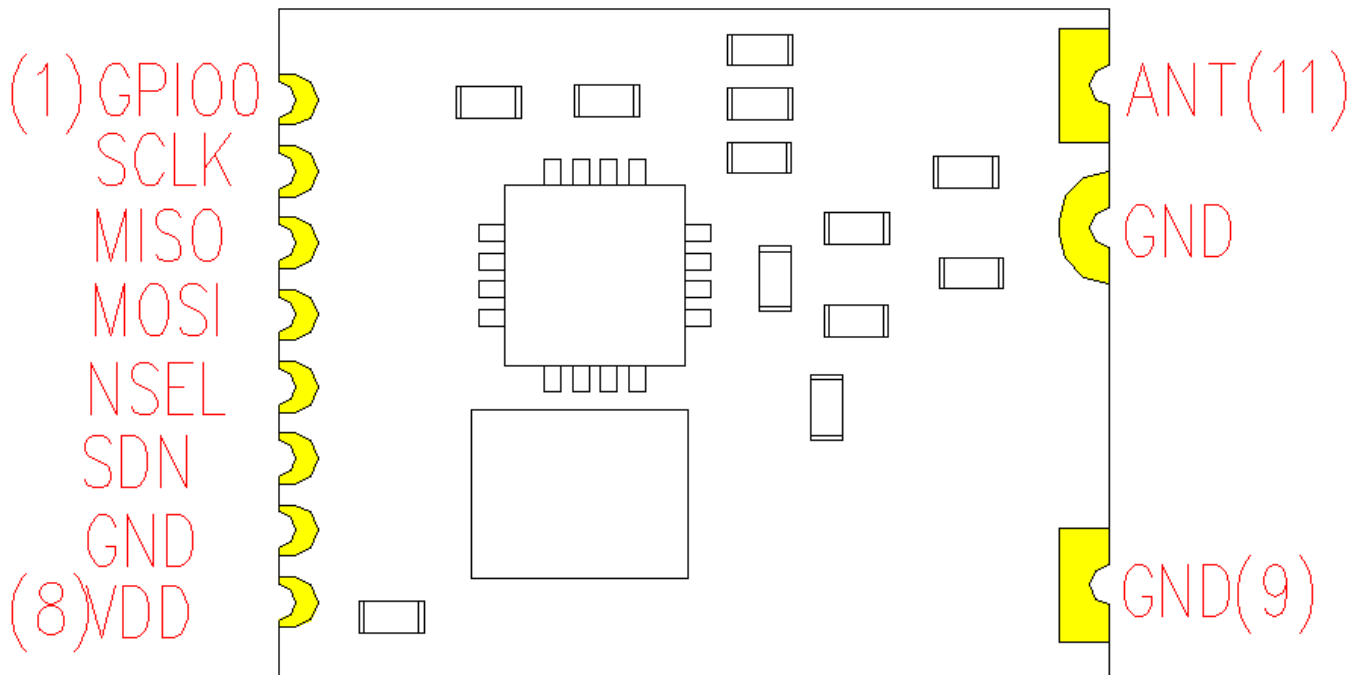
Figure 1. Pinout Top View
