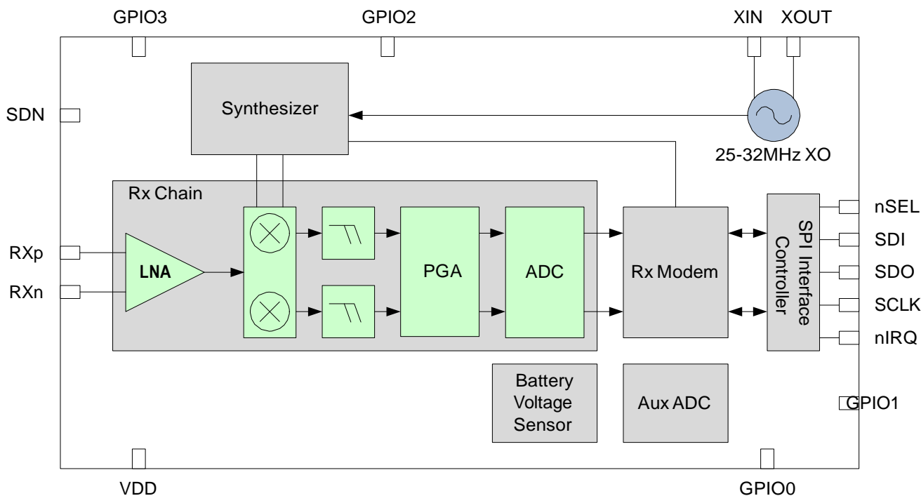
Figure 2. HC4355 Functional Block Diagram
