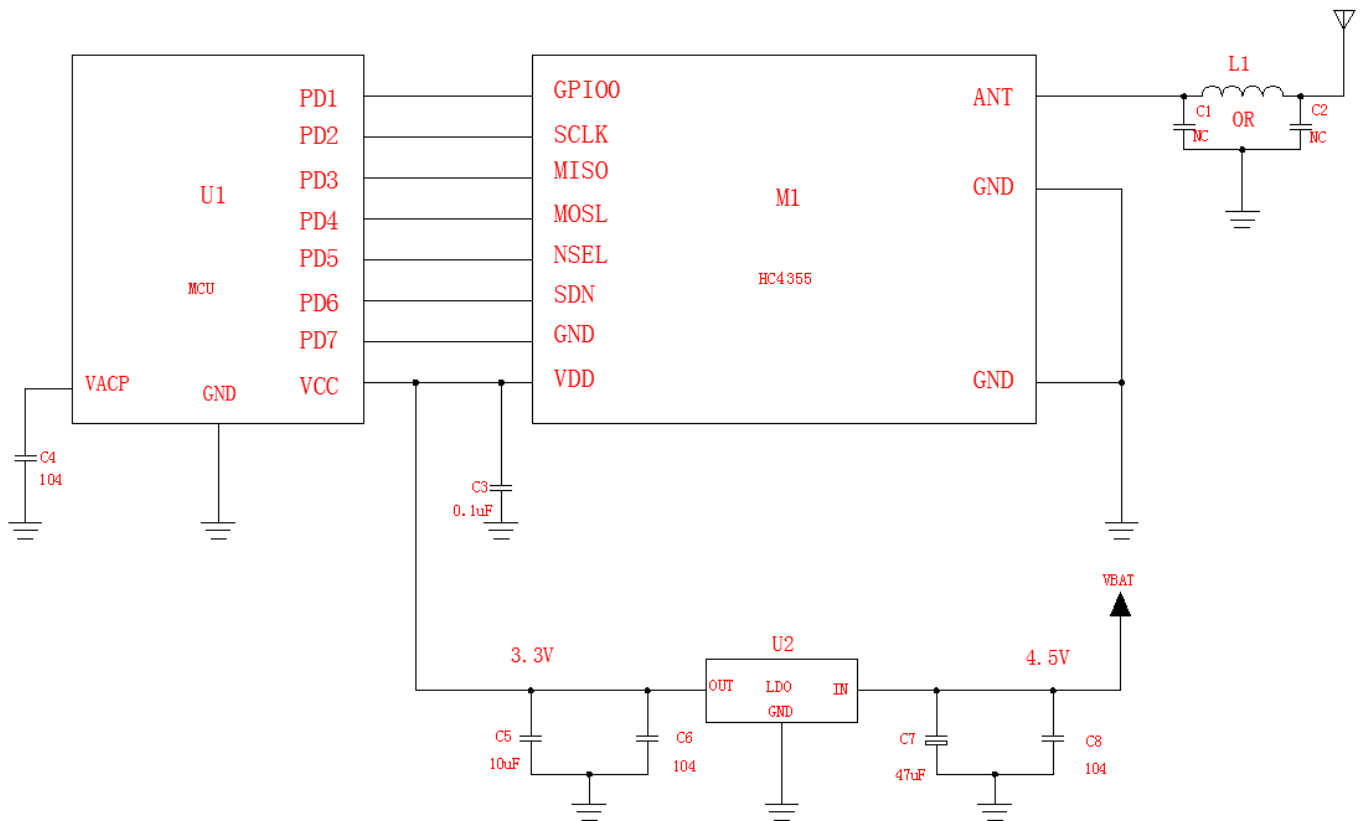
Figure 14. HC4355 Applications Circuit
