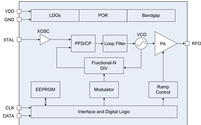
Figure 8. HC216 Functional Block Diagram
