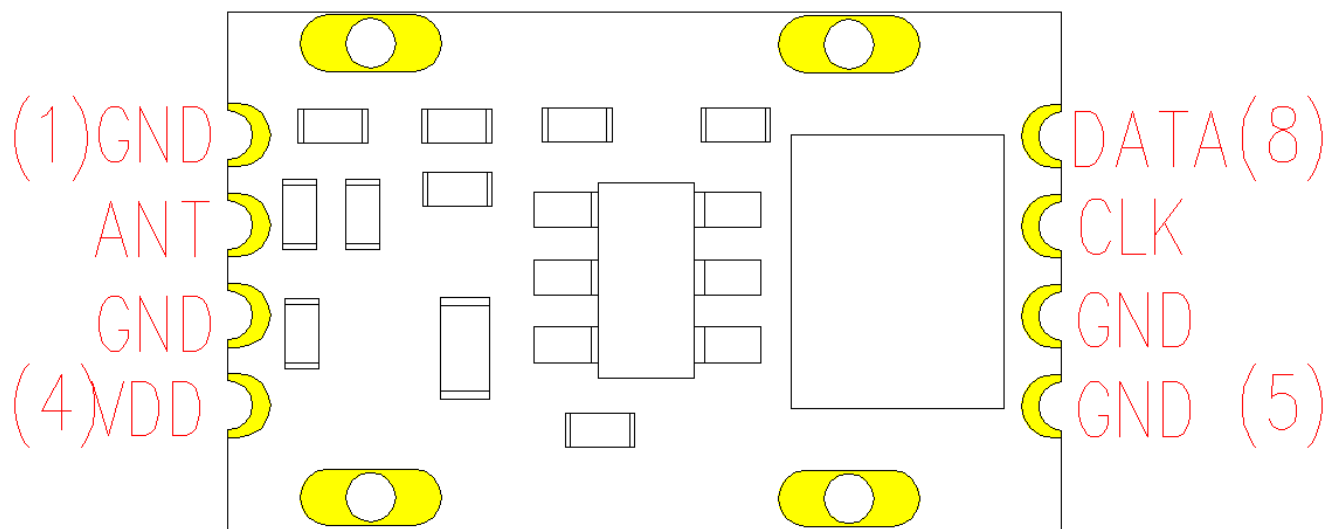
Figure 1. Pin Configuration
