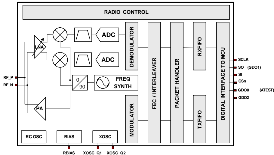
Figure 7: HC210M-TR Simplified Block Diagram
