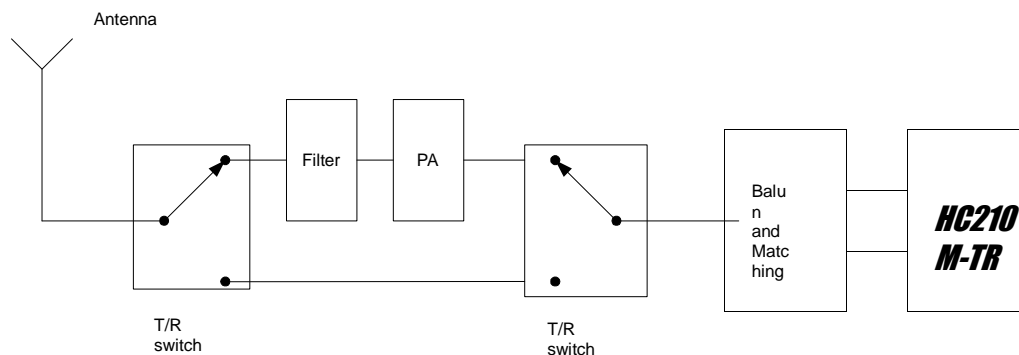
Figure 27: Block Diagram of HC210M-TR Usage with External Power Amplifier
