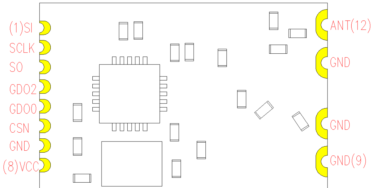
Figure 6: Pinout Top View
