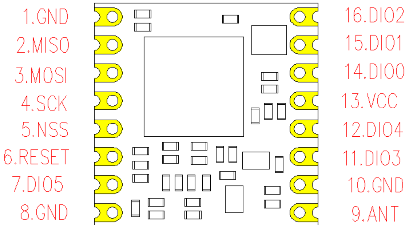
Figure 2. Pin Diagrams
