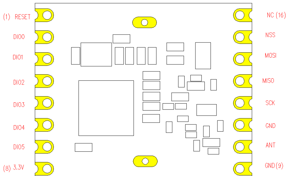
Figure 2. Marking Diagram
