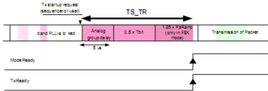
Figure 16. Tx Startup, FSK and OOK
