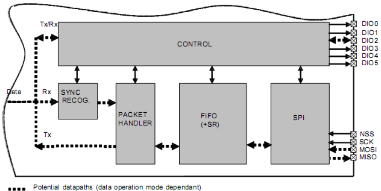
Figure 23. LJ1269C Data Processing Conceptual View
