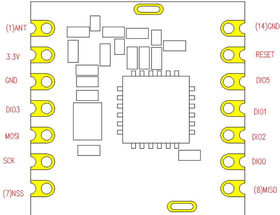
Figure 2. Marking Diagram
