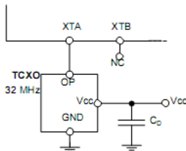
Figure 3. TCXO Connection
