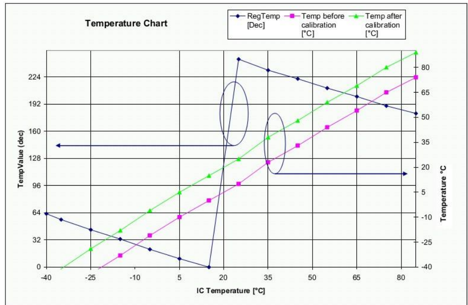
Figure 40. Temperature Sensor Response
