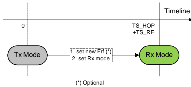
Figure 18. Tx to Rx Turnaround
