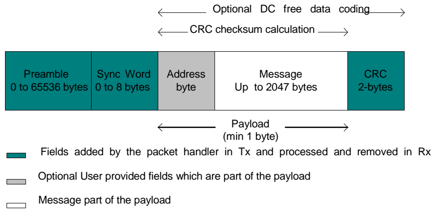
Figure 32. Fixed Length Packet Format
