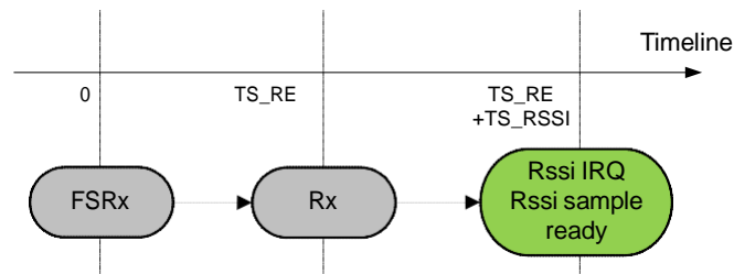
Figure 17. Time to RSSI Sample
