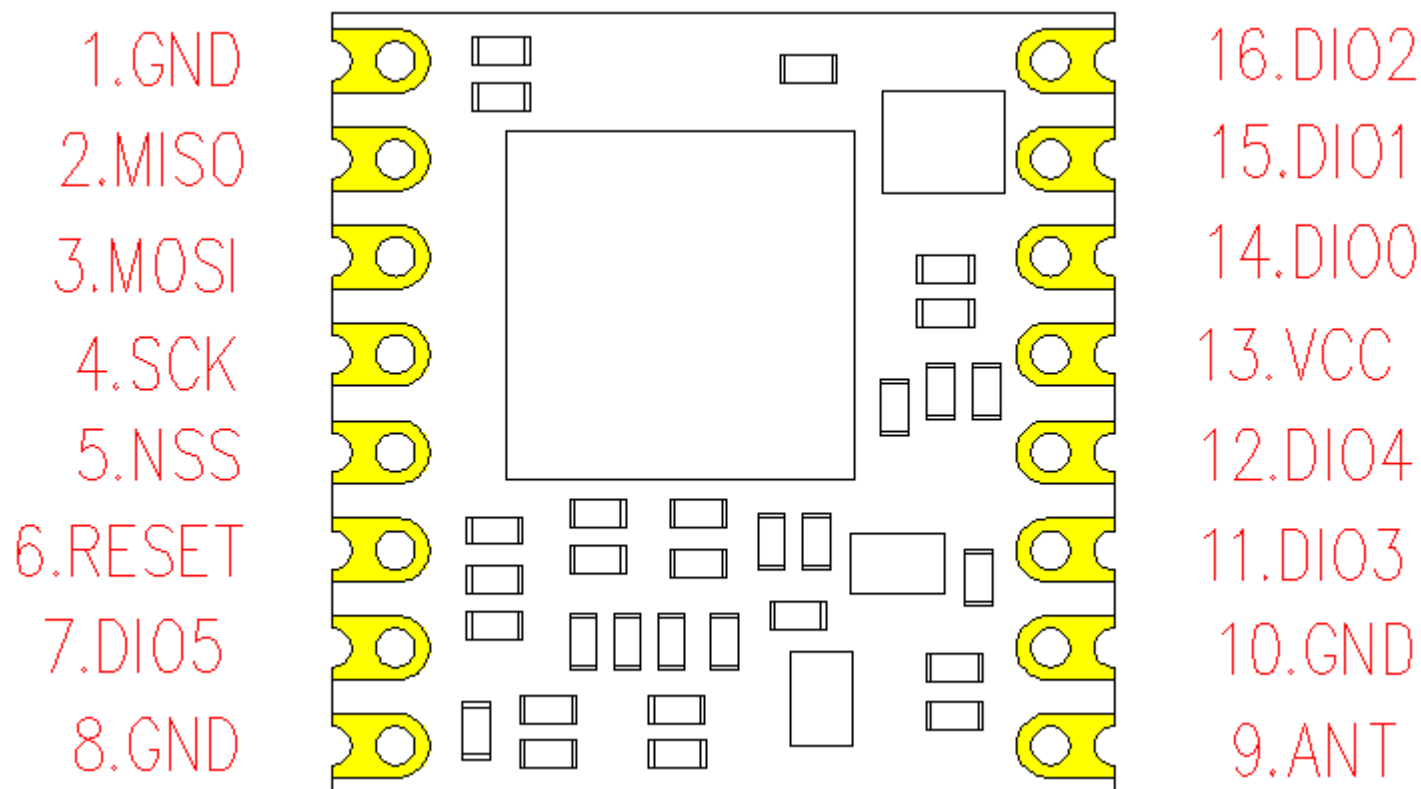
Figure 2. Pin Diagrams
