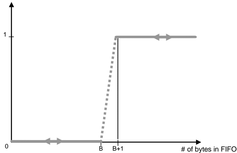
Figure 26. FifoLevel IRQ Source Behavior
