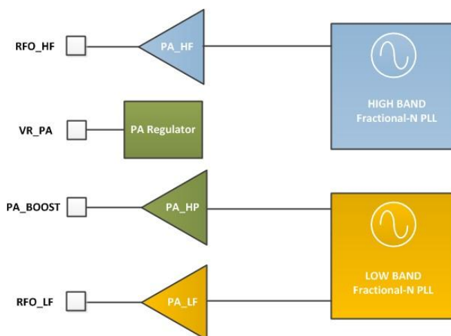
Figure 39. RF Front-end Architecture Shows the Internal PA Configuration.
