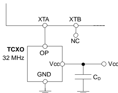
Figure 38. TCXO Connection
