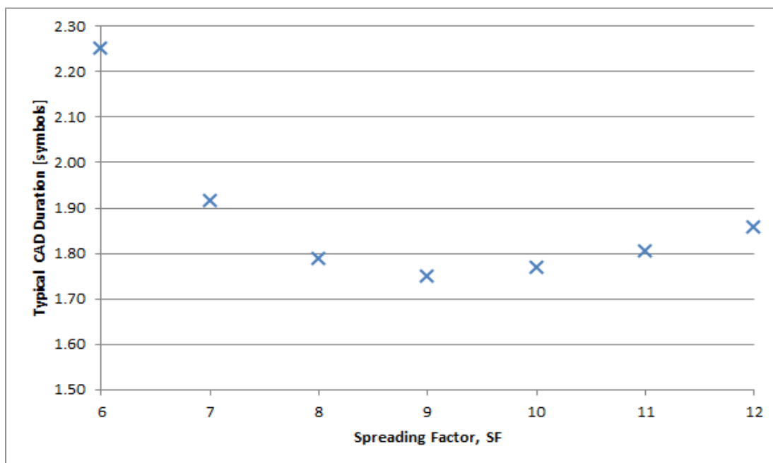
Figure 11. CAD Time as a Function of Spreading Factor
