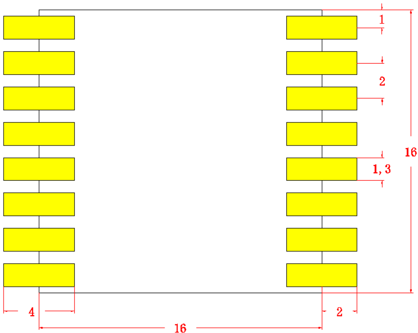
Figure 58. Recommended Land Pattern
