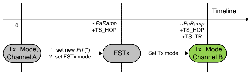
Figure 21. Transmitter Hopping
