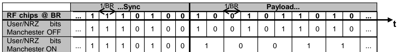
Figure 35. Manchester Encoding/Decoding
