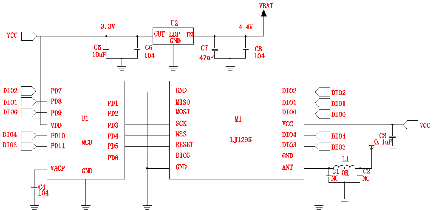
Figure 56 Typical Application Schematic
