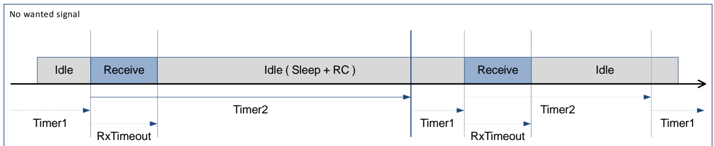
Figure 47. Listen Mode with no SyncAddress Detected
