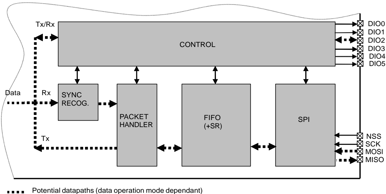
Figure 24. LJ1295/77/78 Data Processing Conceptual View
