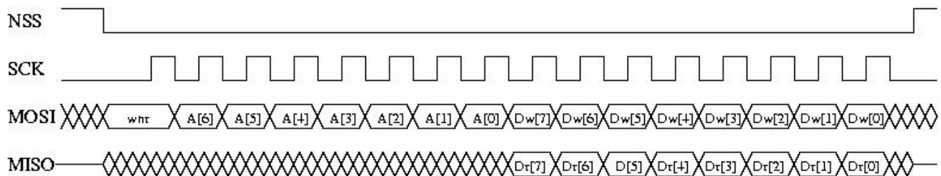
Figure 37. SPI Timing Diagram (single access)
