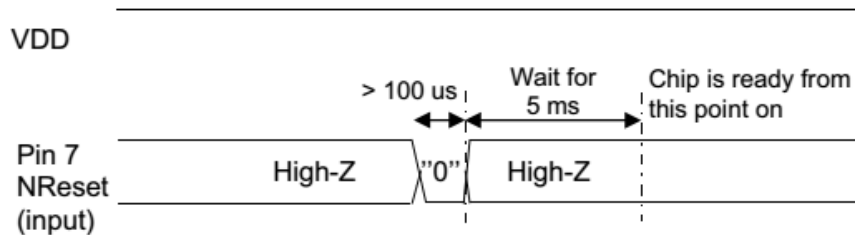
Figure 42. Manual Reset Timing Diagram
