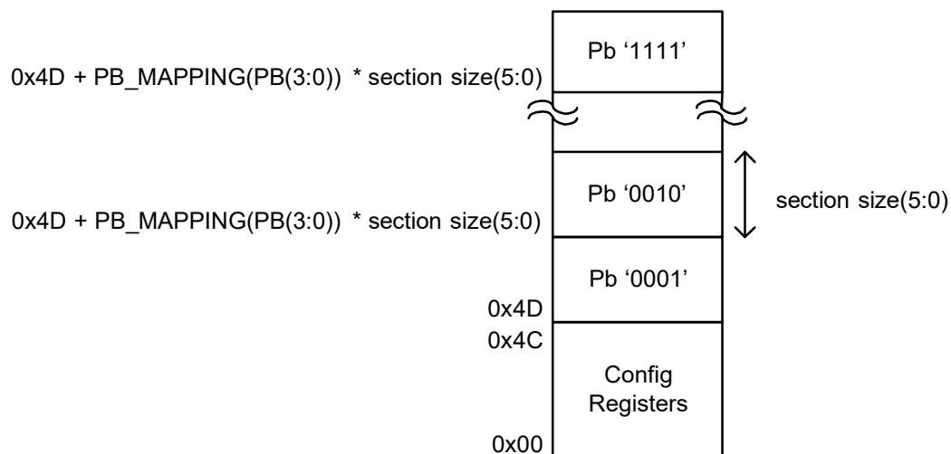
Figure 4. Memory Mapping in Stand Alone Mode
