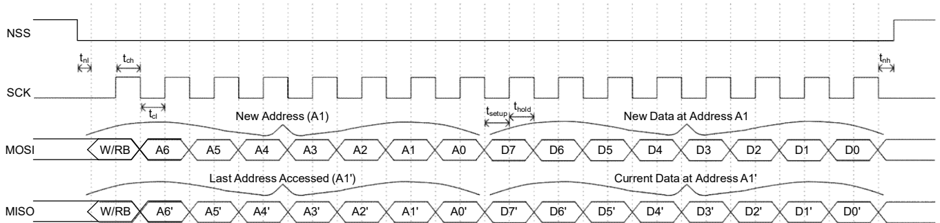
Figure 5. Register Write Access
