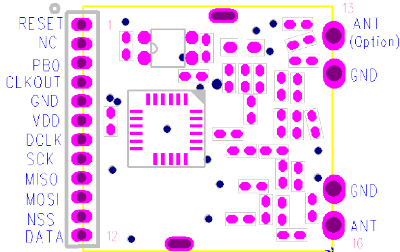
Figure 2. HC1230 Pin diagram (top view)
