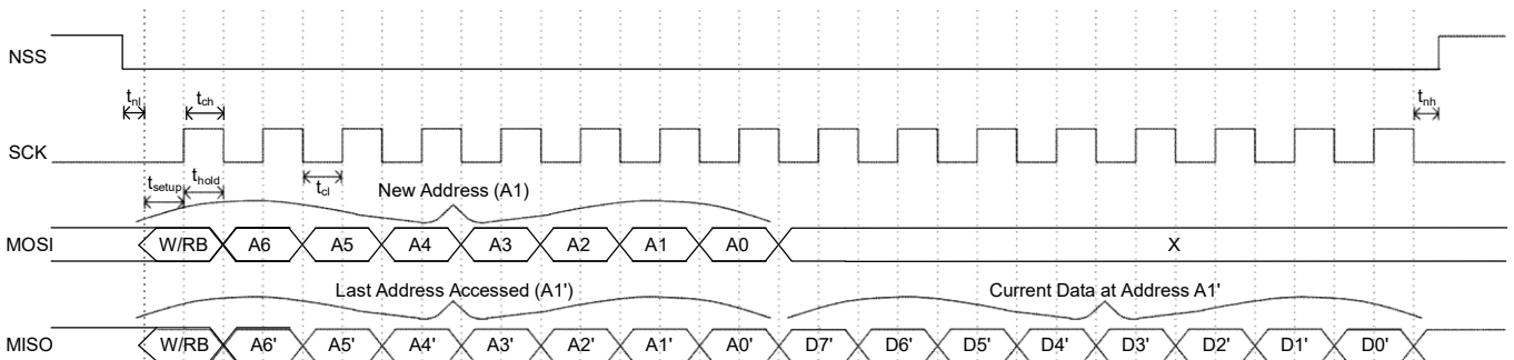
Figure 6. Register Read Access
