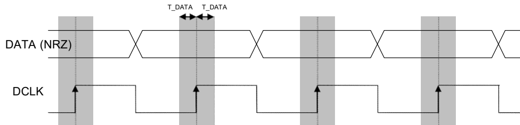
Figure 7. HC1230 Data Clock Timing Diagram (Used Only for Filtering and Ensuring Bit Rate Accuracies)
