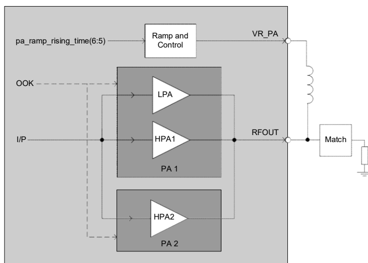
Figure 3. Simplified Schematic of the HC1230 Power Amplifier
